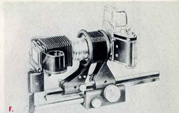
Special duplicating setup for making copies of color and black-and-white transparencies.
