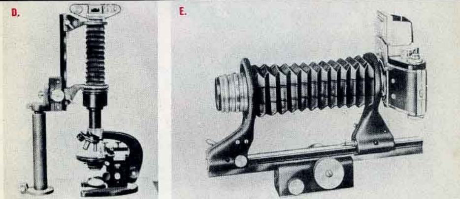
Special duplicating setup for making copies of color and black-and-white transparencies.
